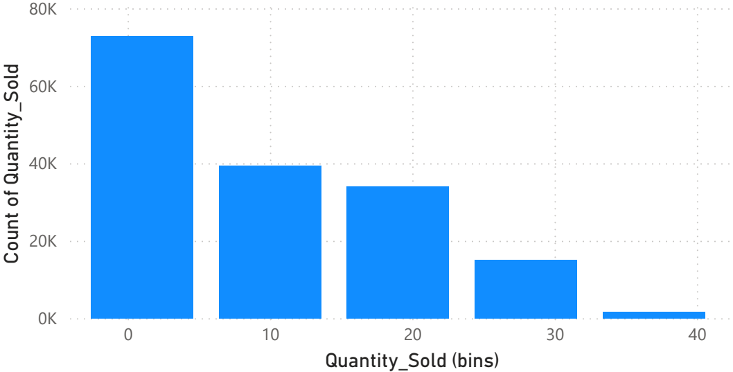
Count of Quantity_Sold by Quantity_Sold (bins)
